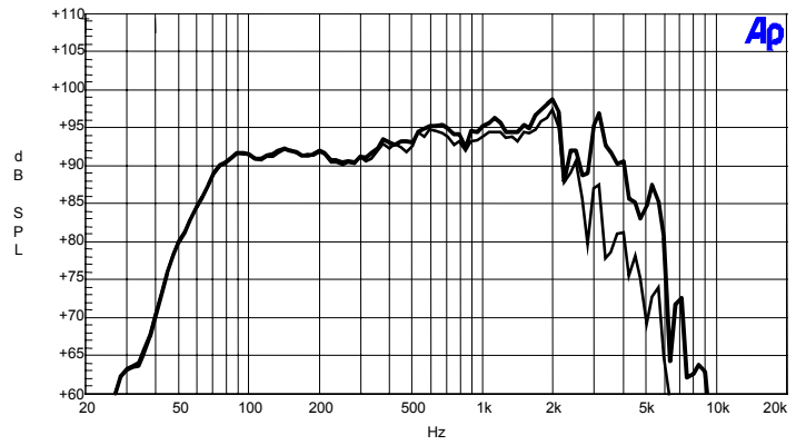
Frequency Response: enclosure volume 35l, port tuning 67Hz (thick curve on axis, thin curve 30° off axis)
