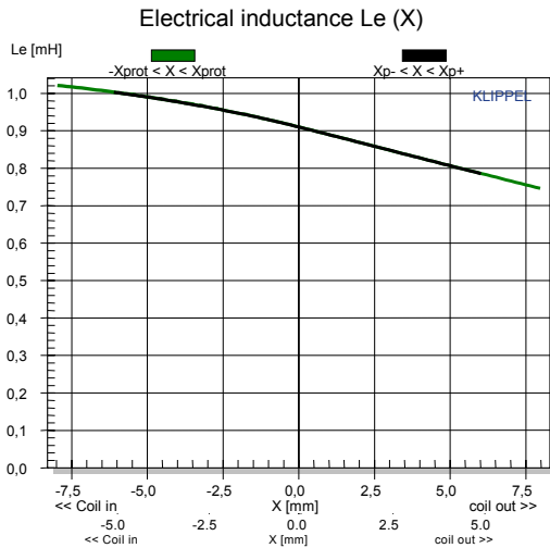
Le : electrical inductance variation with voice coil displacement
